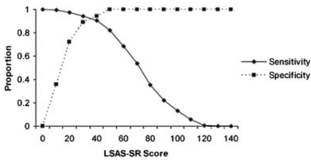
Figure 1. Sensitivity and specificity for classifying participants with social anxiety disorder and nonanxious controls at different values of the LSAS-SR.
