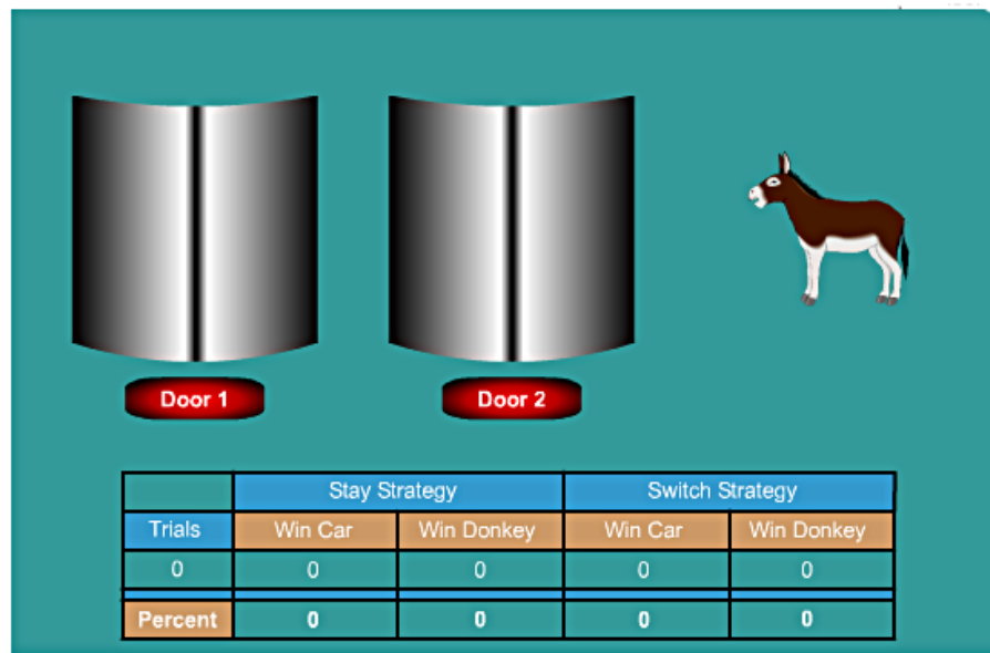
Figure 2: An Animated Simulation Experiment
