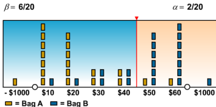
Figure 3: Relating p-values to Type I and II Errors
