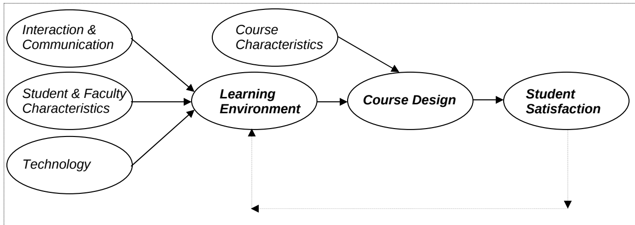
Figure 1: A Framework
