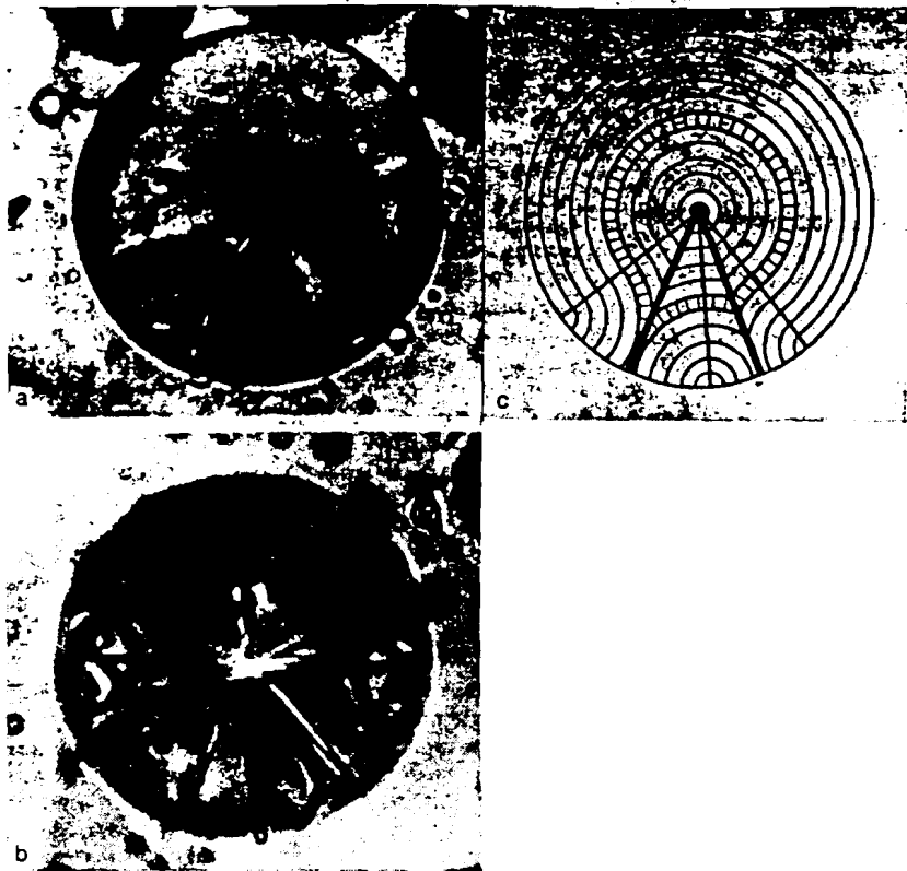
FIG. 3. Structure of spherical smectic-A drops suspended in the glycerine-lecithin matrix M_1 : a,b) microphotographs of drops in transmitted polarized light (the analyzer is absent); c) scheme, corresponding to microphotograph (a), of the packing of the layers in the drop (section through the center of the drop).
