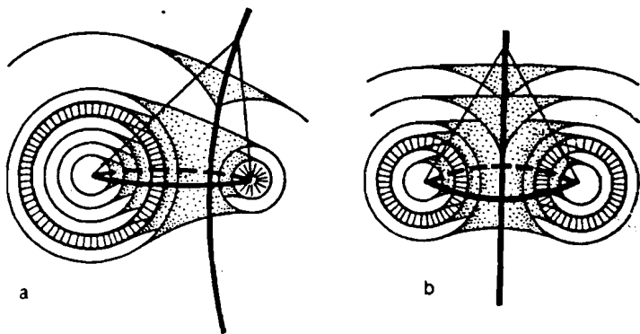
FIG. 1. Smectic-A layers in the form of Dupin cyclides with line defects in the form of a confocal ellipse and hyperbola (a) and a circle-straight-line pair (b). The part of the volume occupied by cyclides and bounded by a surface in the form of a cone of revolution is an isolated confocal domain, whose base is the ellipse (circle) and whose apex lies on the hyperbola (straight line).
