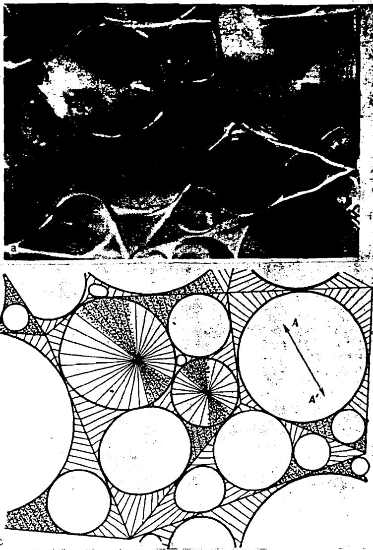
FIG. 5. Polygonal smectic texture in a sample of thickness 200\ \mu\text{m} : a) microphotograph of the upper surface of the texture, in transmitted polarized light with one analyzer; b) the corresponding scheme of the packing of the bases of the confocal domains into polygons—the bases of the pyramids. The distribution of the optical axes on the surface is indicated by the thin straight lines, and the regions of darkening, in which the optical axis is parallel to the plane of polarization of the analyzer, are shaded by dots.
