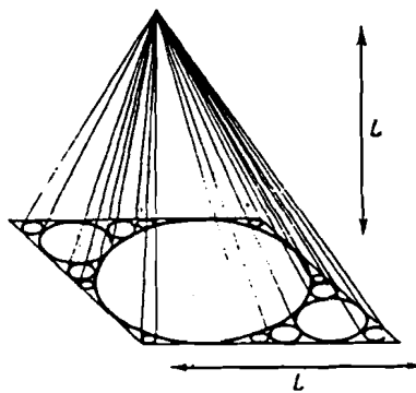
FIG. 2. Iterative filling of a region of space in the form of a pyramid by a family of contiguous confocal domains with a common apex at the apex of the pyramid.
