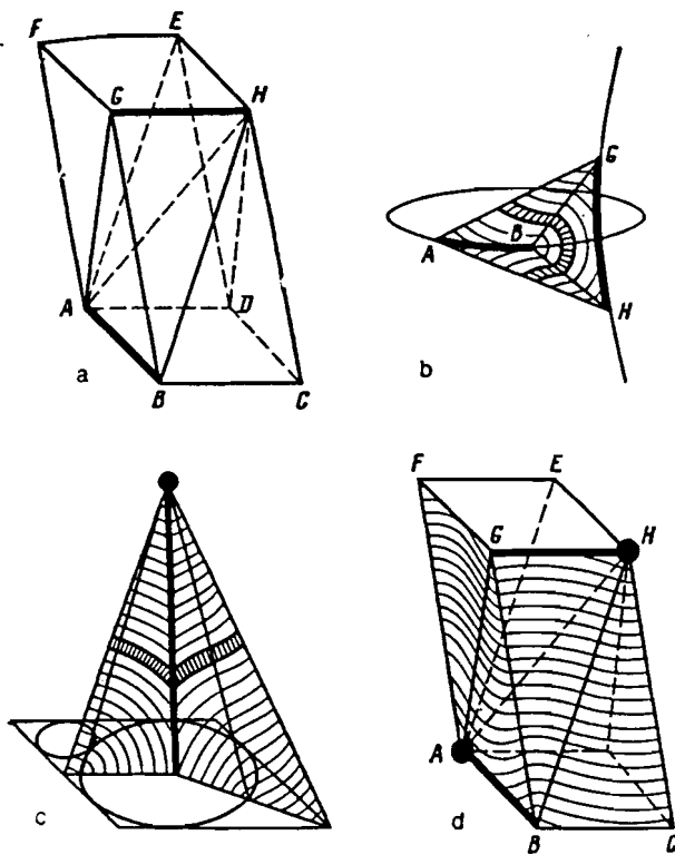
FIG. 6. General scheme of space filling by smectic layers: a) division of a parallelepiped (which can be used to fill space by means of parallel translations) into a pair of pyramids H(ABCD) and A(EFGH) and a pair of tetrahedra ABGH and ADEH ; b) filling of a tetrahedron ABGH by a single family of Dupin cyclides intersecting the faces of the tetrahedron at a right angle; c) filling of a pyramid by a single family of spherical layers, into which confocal domains are built smoothly; d) scheme of a smooth crossing of layers from a pyramid to a tetrahedron within one parallelepiped.
