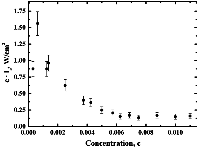
FIGURE 3 Product I_c(c) \cdot c vs. c ; homeotropic 10 \mu m cell.
