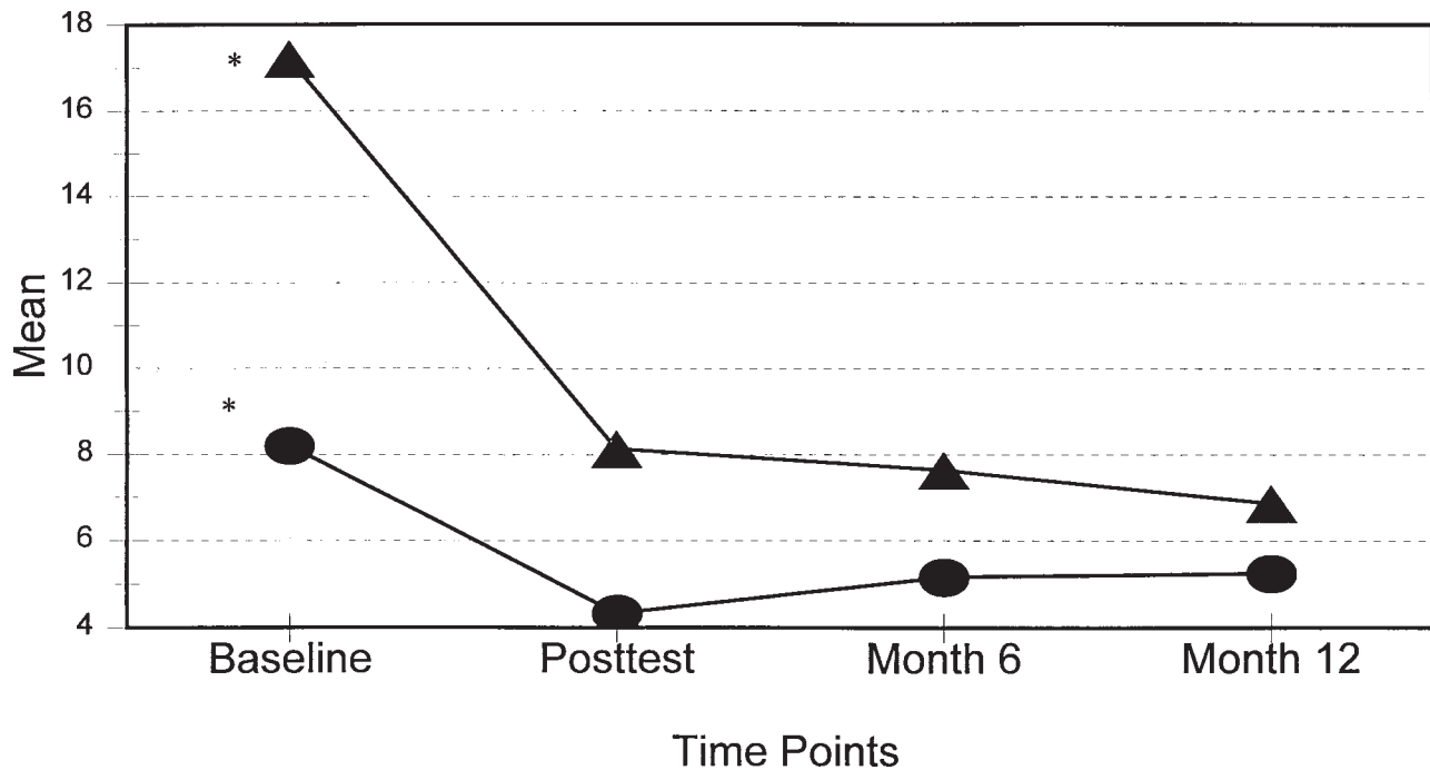
Figure 2. Observed means of LSAS social fear for completers in generalized (GEN) and non-generalized (NGEN) subtypes
