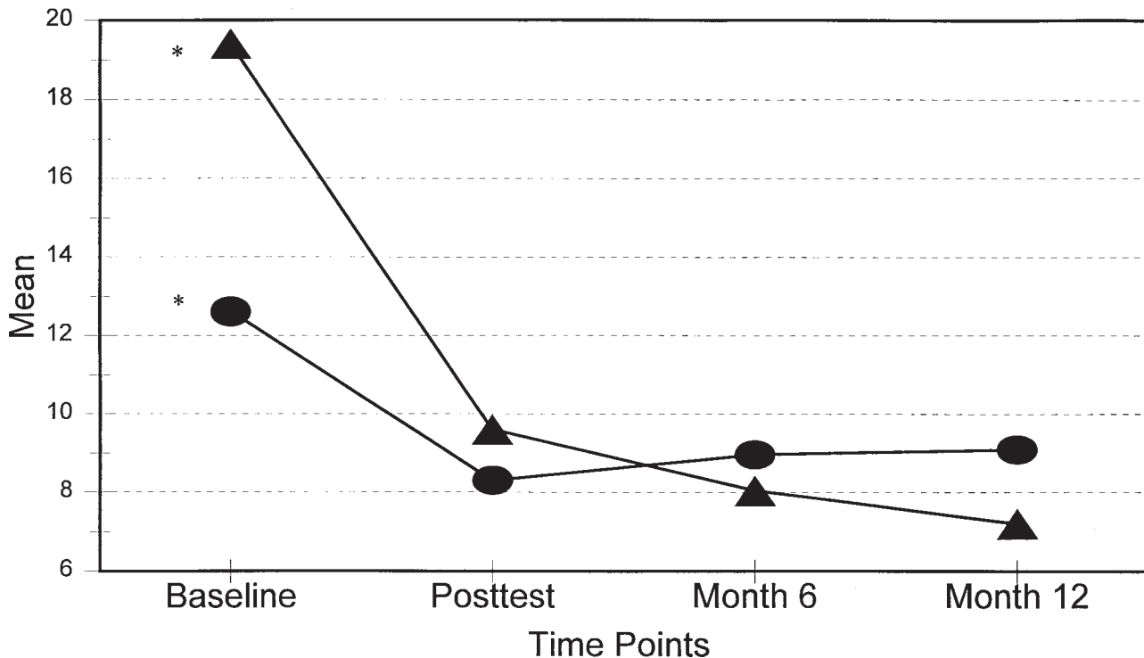
Figure 1. Observed means of LSAS performance fear for completers in generalized (GEN) and non-generalized (NGEN)
