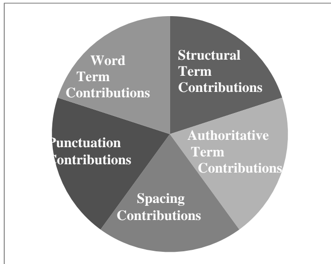
Figure 1. Contribution Rubric
