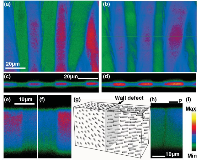
FIG. 2 (color). (a),(b) In-plane and (c),(d) vertical FCPM cross sections of the director structure in a relatively thin ring; (e),(f) vertical FCPM cross sections obtained for a thick ring illustrating that orientation of \hat{n} across the film thickness is the same within the stripes; (g) schematics of DNA orientation (visualized by cylinders) in domains with \hat{n} at \approx \pm 45^\circ to the radial direction and the vertical wall defect (shaded plane) in between; (h) a typical FCPM vertical cross section of a thick ring (FCPM polarization along the local CL) visualizes the wall defect separating domains with nearly orthogonal \hat{n} ; (i) FCPM intensity scale. The polarization of the FCPM probing light is at -45^\circ with respect to the radial direction in (a),(c),(e) and at 45^\circ in (b),(d),(f).
