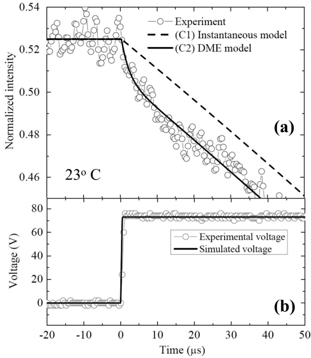
FIG. 8. Normalized transmitted light intensity (a) and voltage (b) versus time for the mixture 53.7 wt. % MLC7026-100 +46.3 wt. % MLC2048 driven by a fast-changing rectangular pulse. The circles are the experimental data; the curves represent simulations with different models as indicated by the labels.
