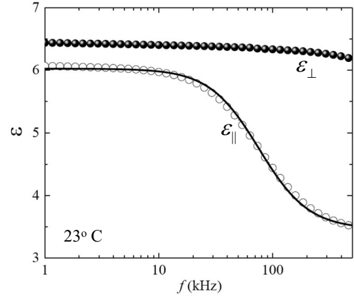
FIG. 7. Dielectric dispersion curves for the real components ( \varepsilon_{\parallel} , \varepsilon_{\perp} ) of the mixture 53.7 wt. % MLC7026-100+46.3 wt. % MLC2048 at 23 °C. The solid curve is fitted with Eq. (24) where \varepsilon_{f\parallel} = 3.5 , \varepsilon_{f\parallel} = 6.0 , and \tau_{\parallel} = 2.1 \mu\text{s} .
