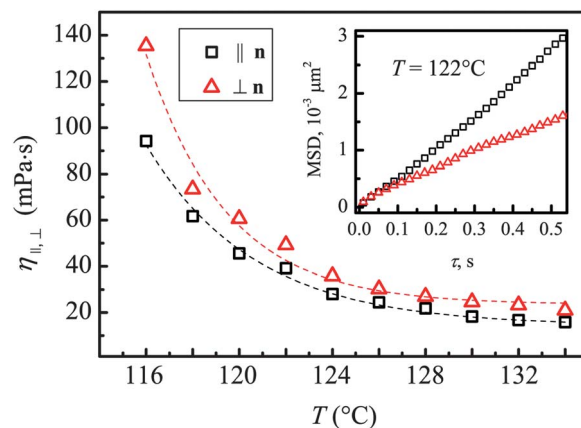
Fig. 8 Flow viscosities \eta_{\parallel} and \eta_{\perp} for 12-F as a function of temperature. The inset shows a typical mean-square displacement (MSD) of the probe particle vs. time at 122 °C.
