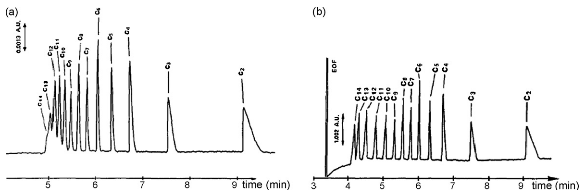
Fig. 2 – Effect of addition of a \beta -CD derivative on the separation of C_2 – C_{14} linear FFA standard mixture ( 0.5 \text{ mmol L}^{-1} each in methanol) in a purely aqueous electrolyte. Fused-silica capillary, 50 \mu\text{m} I.D. \times 72 cm (50 cm to detector). Electrolyte, 20 \text{ mmol L}^{-1} Tris– 10 \text{ mmol L}^{-1} p -anisate (pH 8.2): (a) without any additive; (b) with 0.75 \text{ mmol L}^{-1} trimethyl- \beta -CD added. Applied voltage, 30 kV ( I = 3 \text{ A} ). Temperature, 30^\circ\text{C} . Indirect absorbance detection at 270 nm. Hydrodynamic injection for 1 s. EOF = electro-osmotic flow. Adapted with permission from [41].
