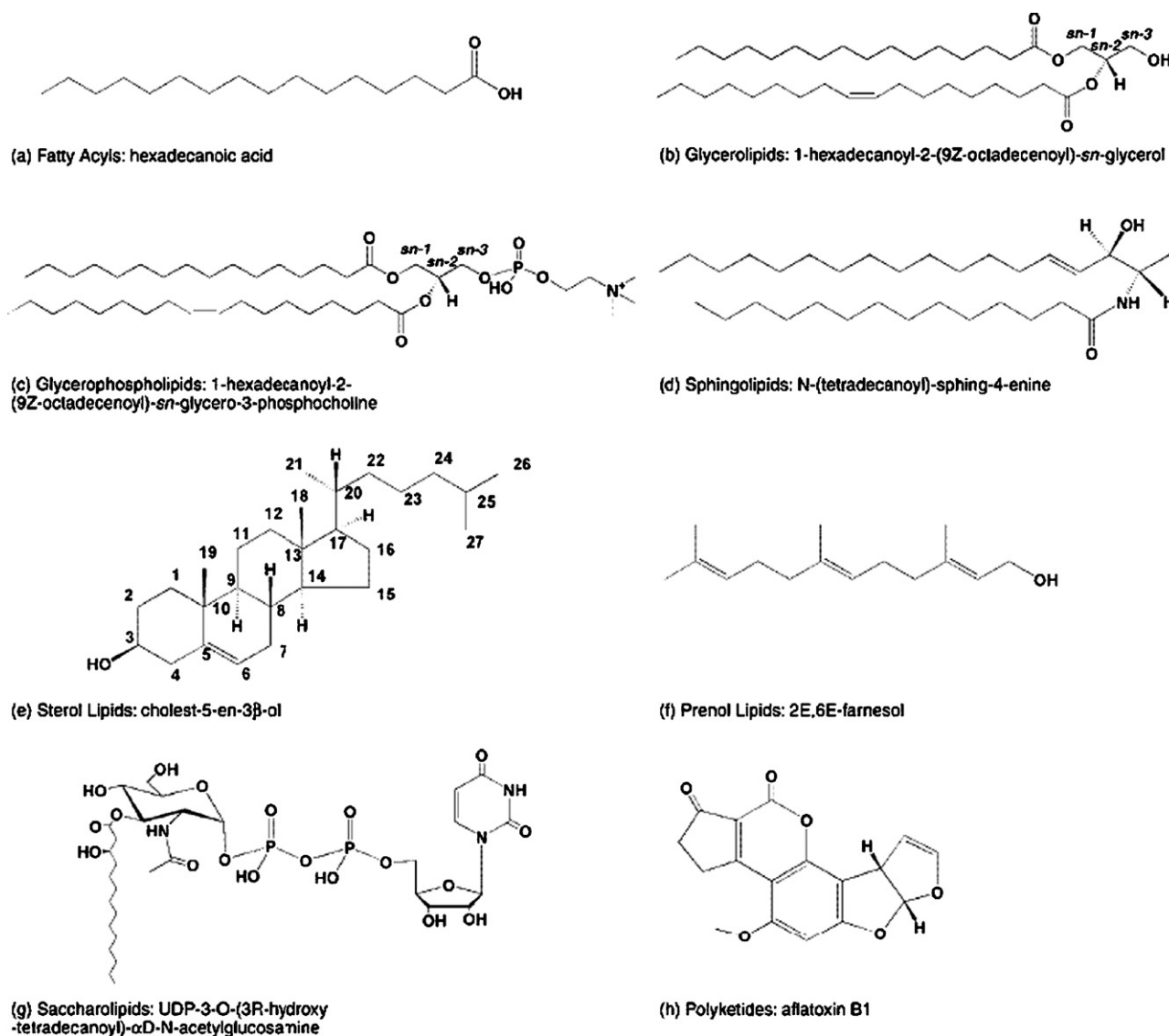
Fig. 1 – Representative structures for each lipid category. Adapted with permission from [3].
