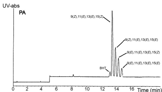
Fig. 4 – Separation of underivatized 9,11,13,15-octadecadienoate isomers ( \alpha -parinaric acid and its geometrical isomers). Conditions: capillary, fused silica 50 \mu m I.D., effective length 50 cm (total length 58 cm); 30 kV; 20 \mu A; 15 °C. Background electrolyte, 40 mM borate (pH 9.20), 4 M urea, 15 mM SDS, 20% MeOH (v/v); detection: UV at 305 nm. BHT = butylated hydroxytoluene. Adapted with permission from [76].
