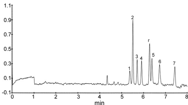
Fig. 3 – Typical electropherogram of carnitine and short-chain acylcarnitines standards. The concentrations are 100 \text{ mM} for carnitine/acylcarnitines and 50 \text{ mM} for the internal standard. The final preparation was diluted 10 times before injection. Capillary electrophoresis buffer and additives were 20 \text{ mM} \text{NaH}_2\text{PO}_4 , 20 \text{ mM} \text{H}_3\text{PO}_4 and 20 \text{ mM} SDS in acetonitrile–water (50:50, v/v). The peaks are: (1) internal standard, (2) carnitine, (3) acetylcarnitine, (4) propionylcarnitine, (5) isovaleryl carnitine, (6) hexanoyl carnitine, (7) octanoyl carnitine and (r) peak from the derivatizing agent. UV detection at 260 nm. Adapted with permission from [63].
